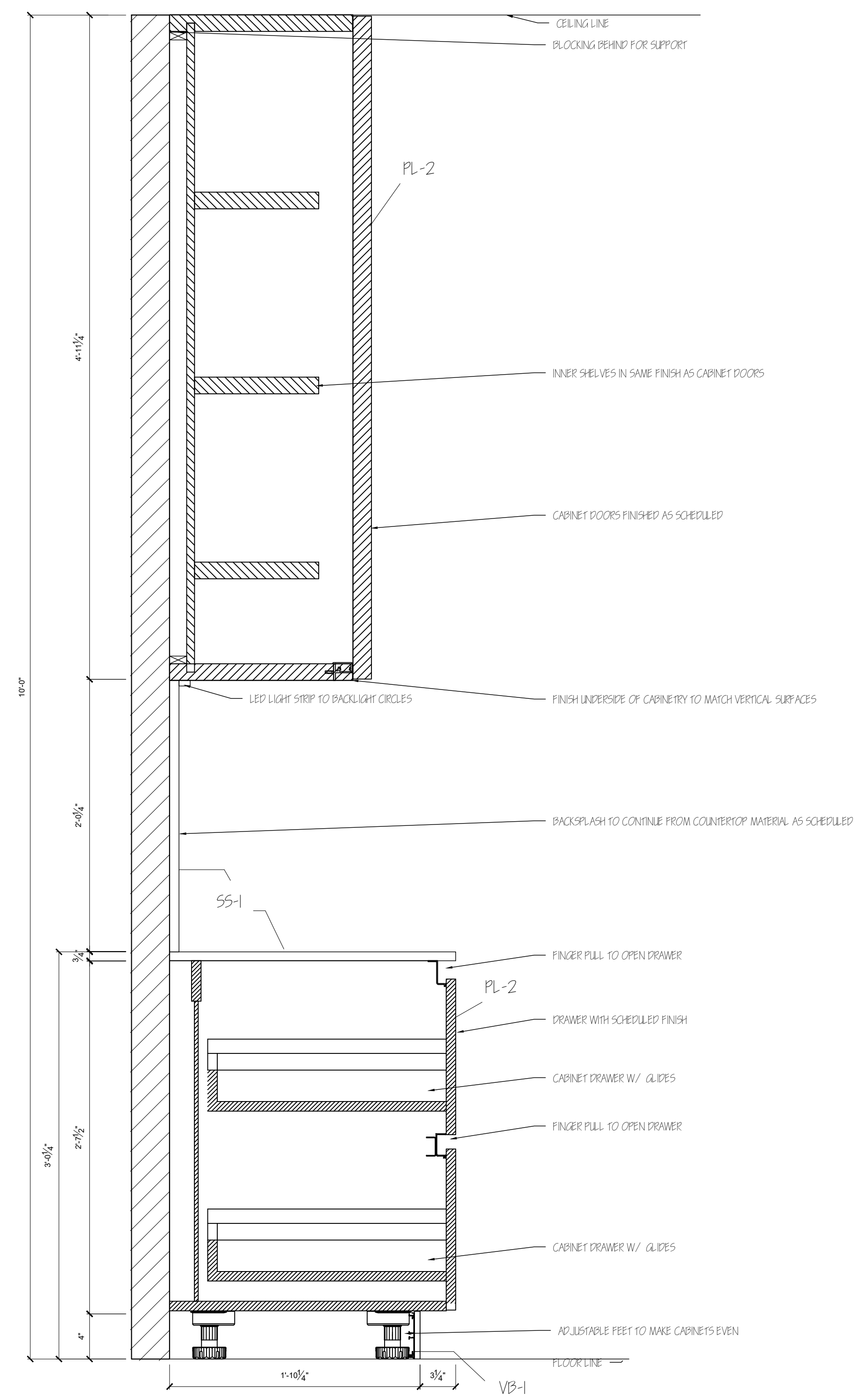
1 BREAK ROOM I MILLWORK DETAIL SCALE: \frac{1}{2} " = 1'-0"
