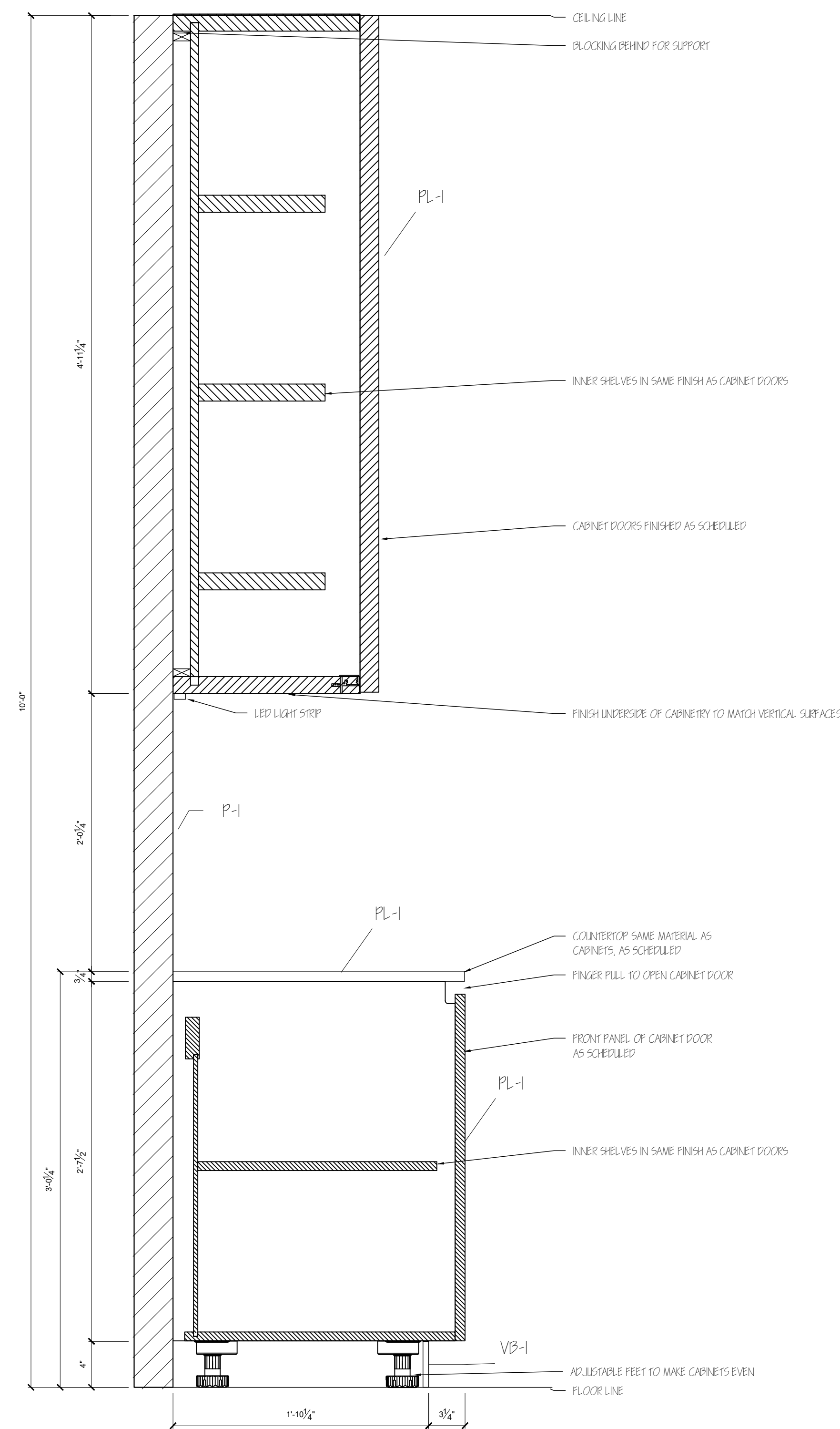
2 COPY ROOM MILLWORK DETAIL - TYPICAL SCALE: \frac{1}{2} " = 1'-0"
