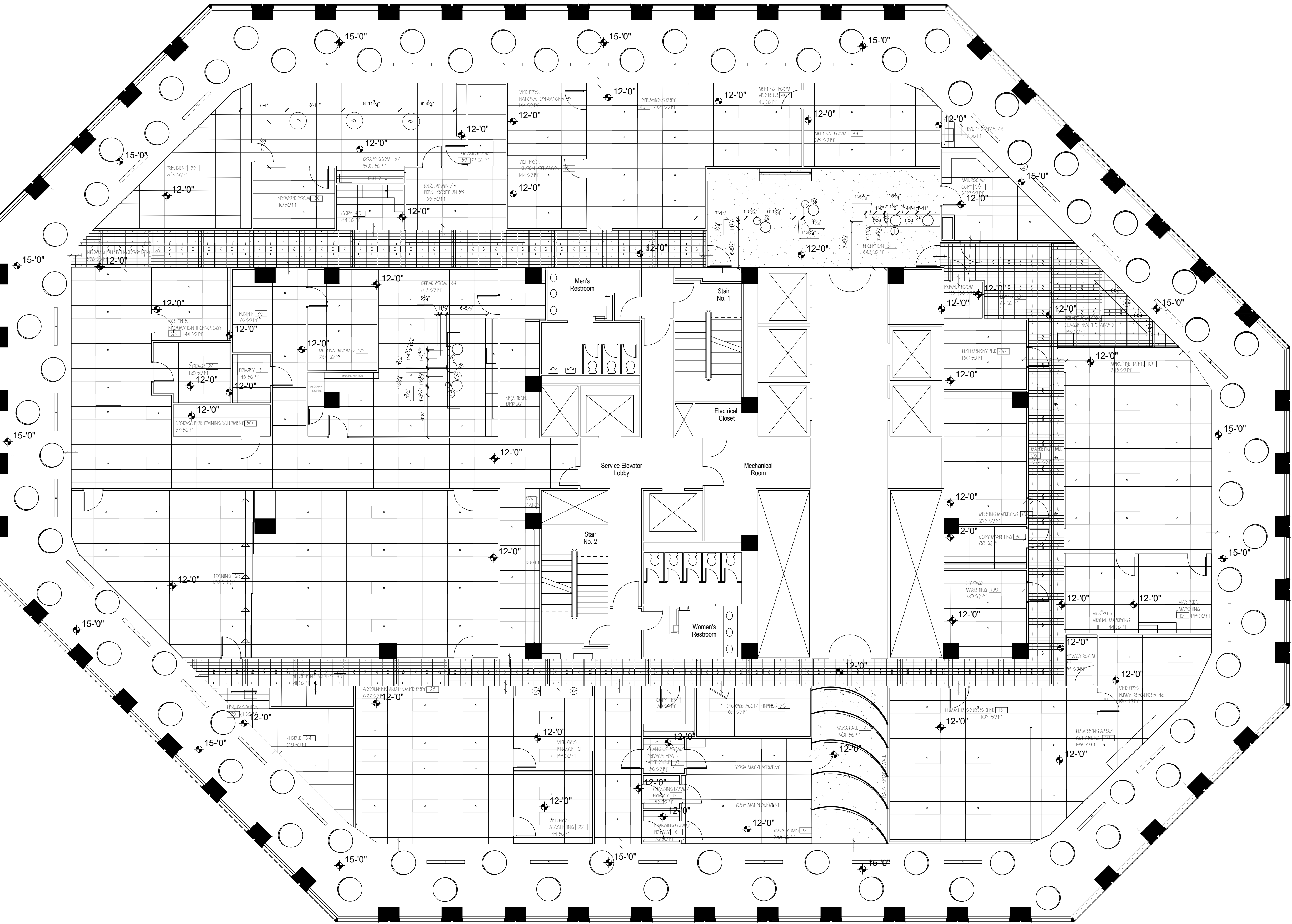
1 REFLECTED CEILING PLAN SCALE: 1/8" = 1'-0"
