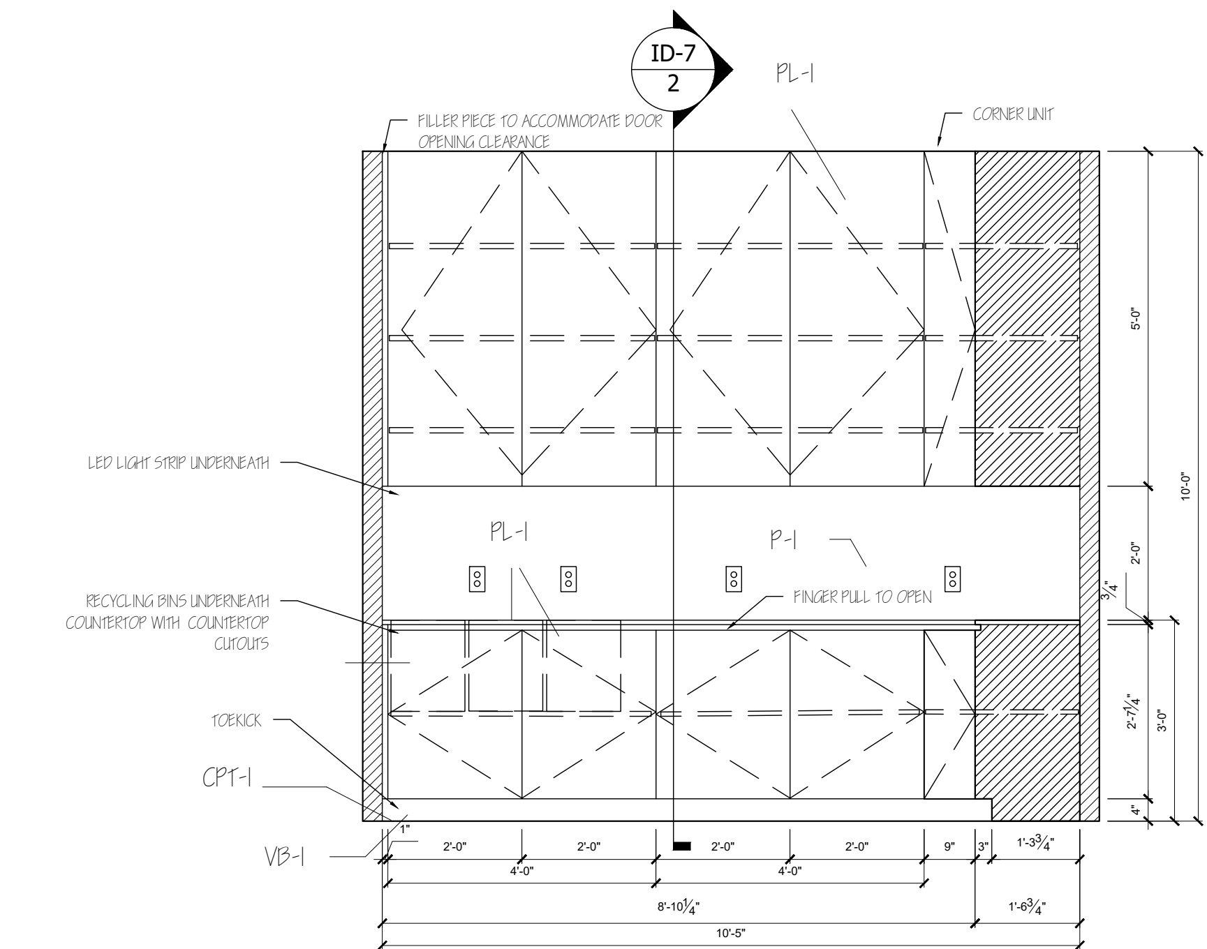
5 COPY ROOM #40 ELEVATION SCALE: 1/2" = 1'-0"
