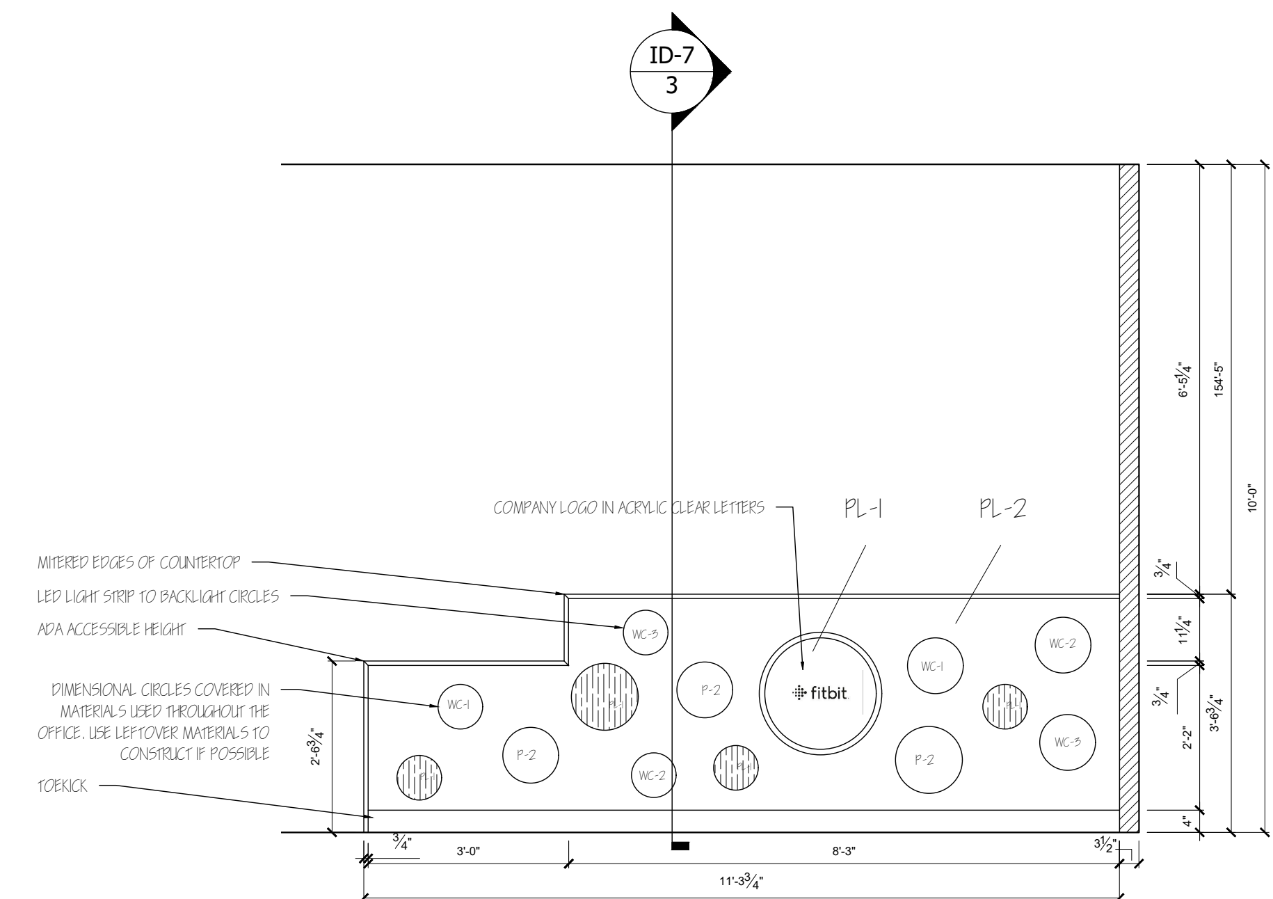
2 RECEPTION DESK #1 ELEVATION SCALE: 1/2" = 1'-0"
