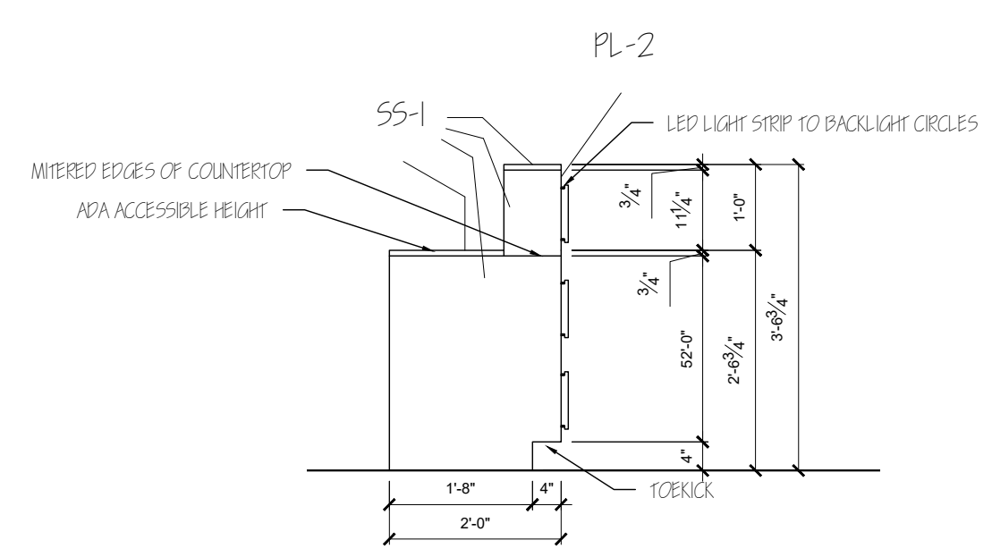
3 RECEPTION DESK #1 SIDE ELEVATION SCALE: 1/2" = 1'-0"
