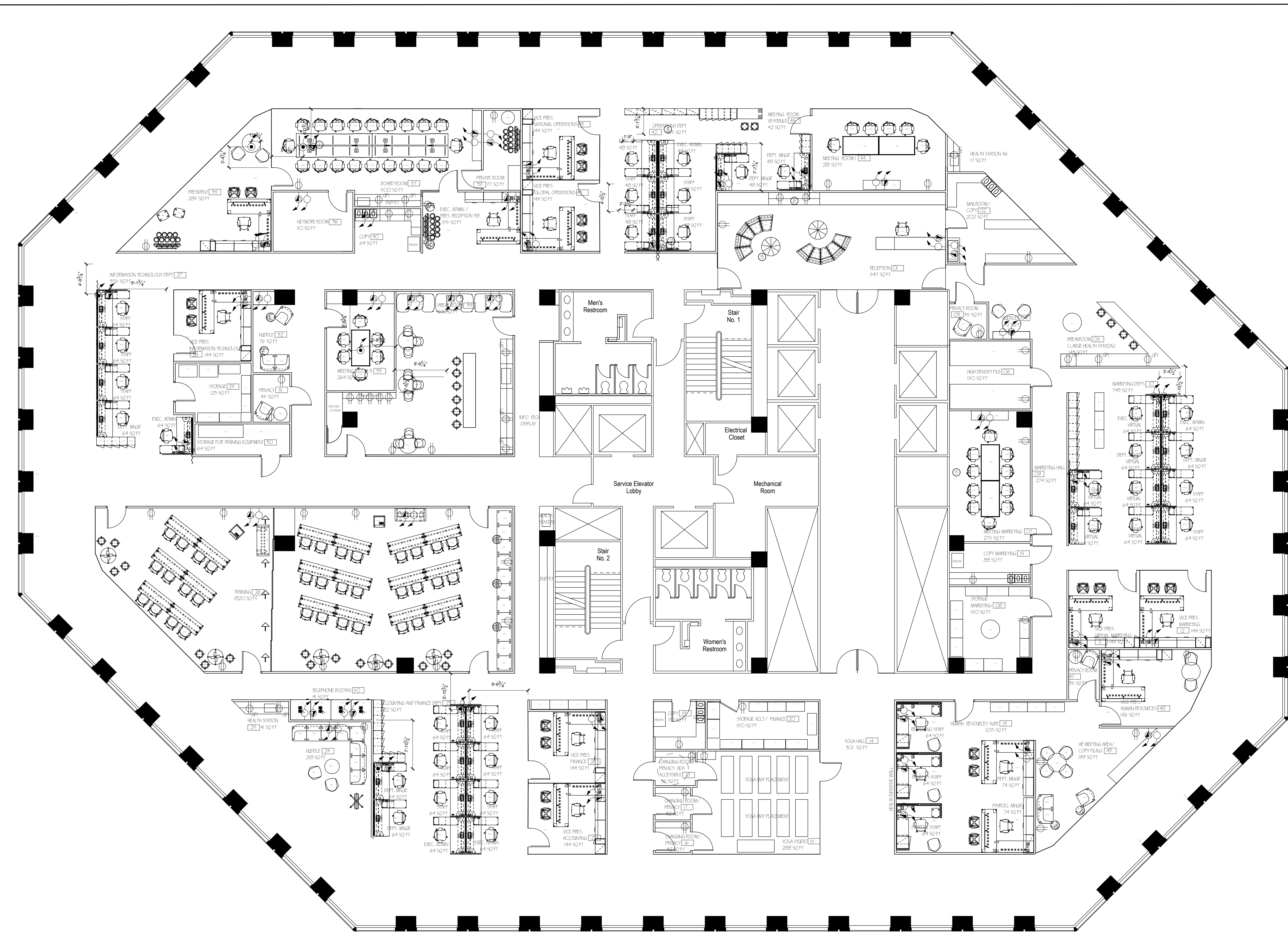
1 FURNITURE AND POWER PLAN SCALE: 1/8" = 1'-0"
