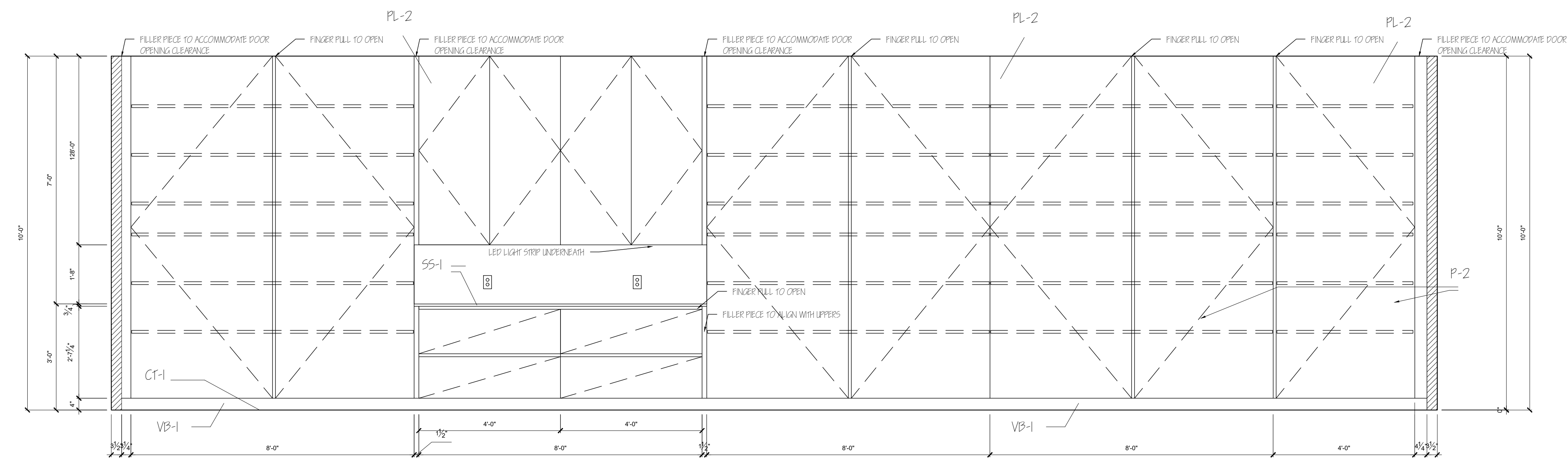
1 RECEPTION ROOM #1 ELEVATION SCALE: 1/2" = 1'-0"
