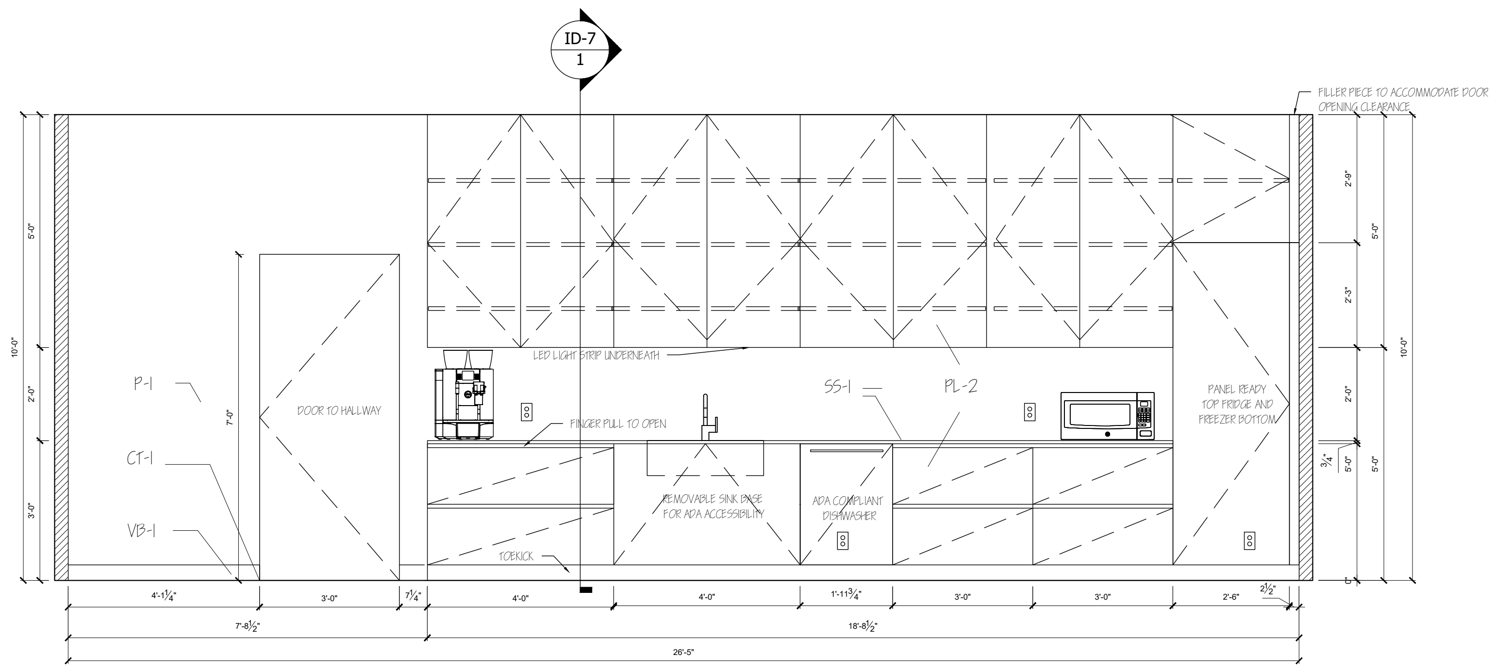
4 BREAK ROOM I #30 ELEVATION SCALE: 1/2" = 1'-0"
