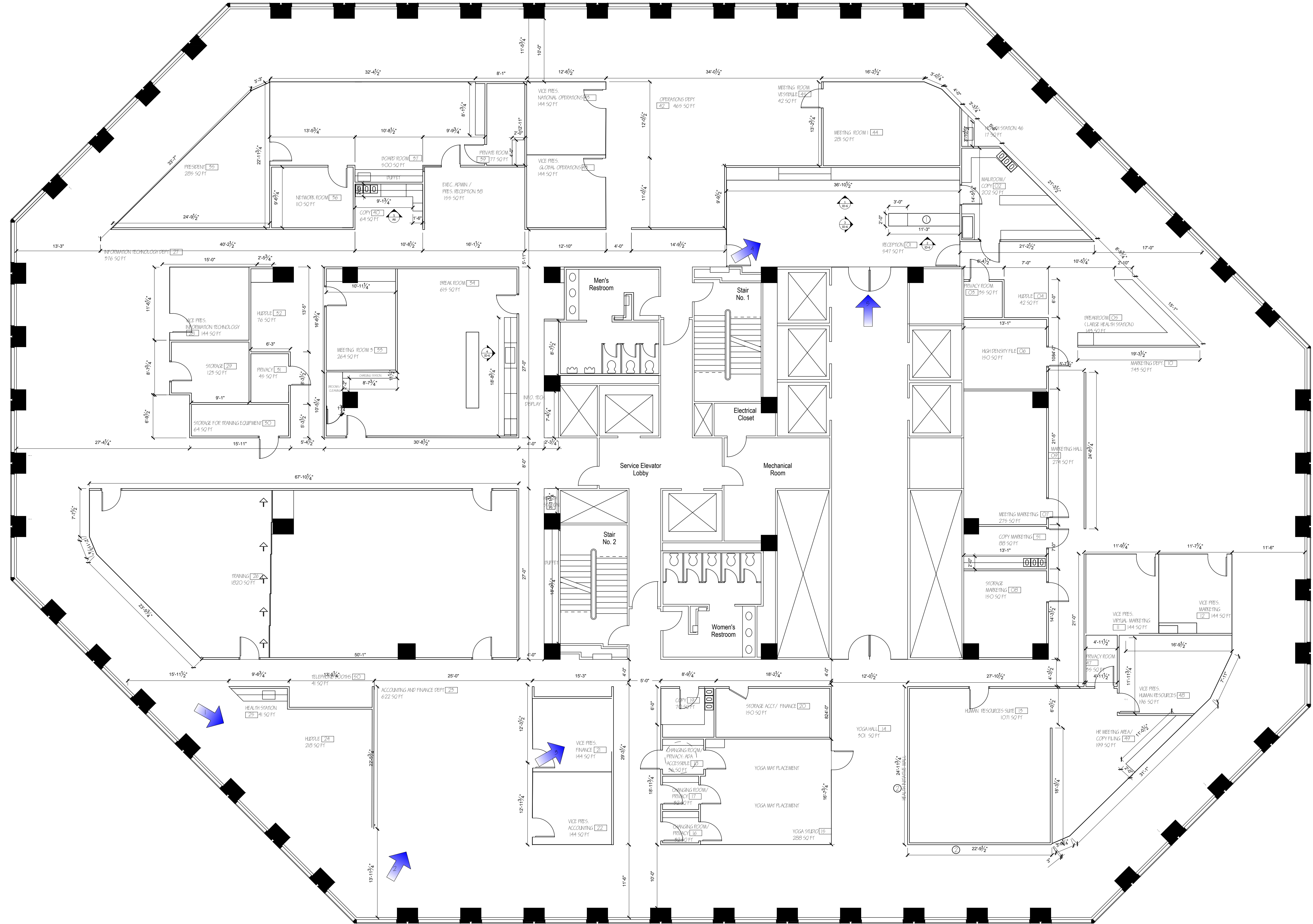
1 ARCHITECTURAL FLOOR PLAN SCALE: 1/8" = 1'-0"
