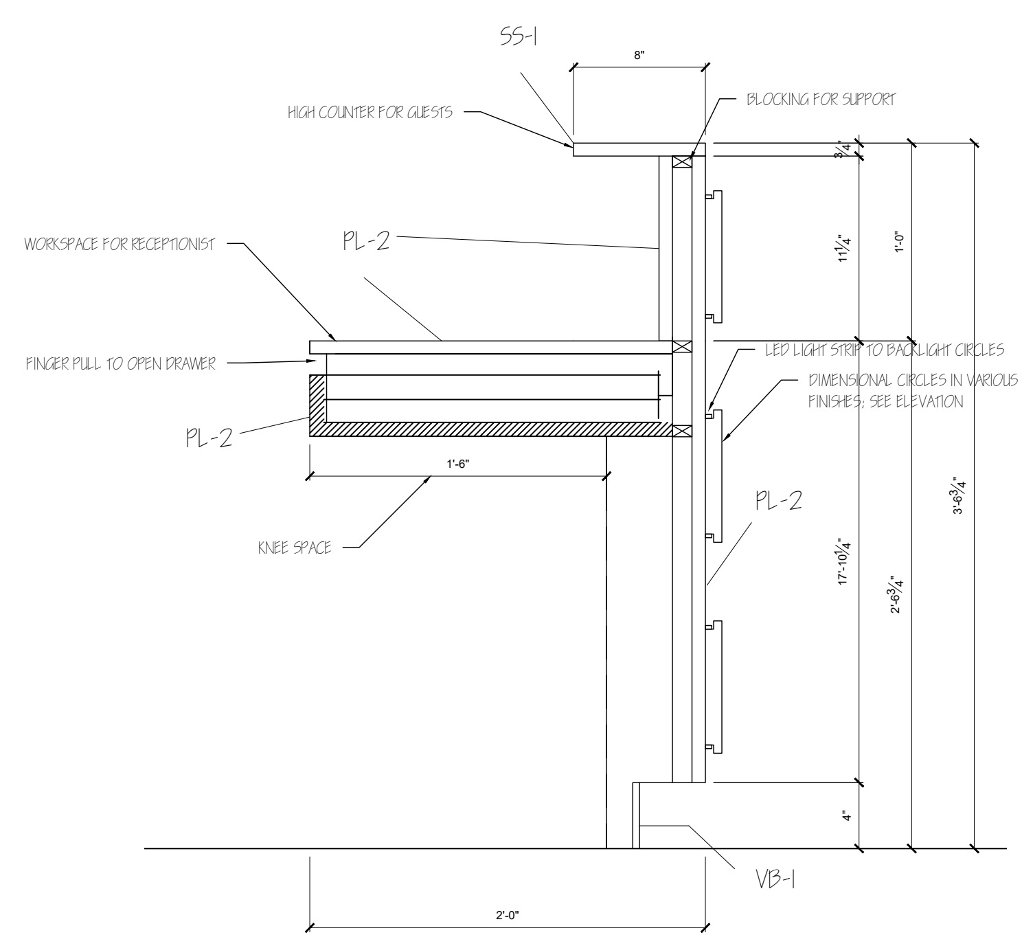
3 RECEPTION DESK MILLWORK DETAIL SCALE: \frac{1}{2} " = 1'-0"
