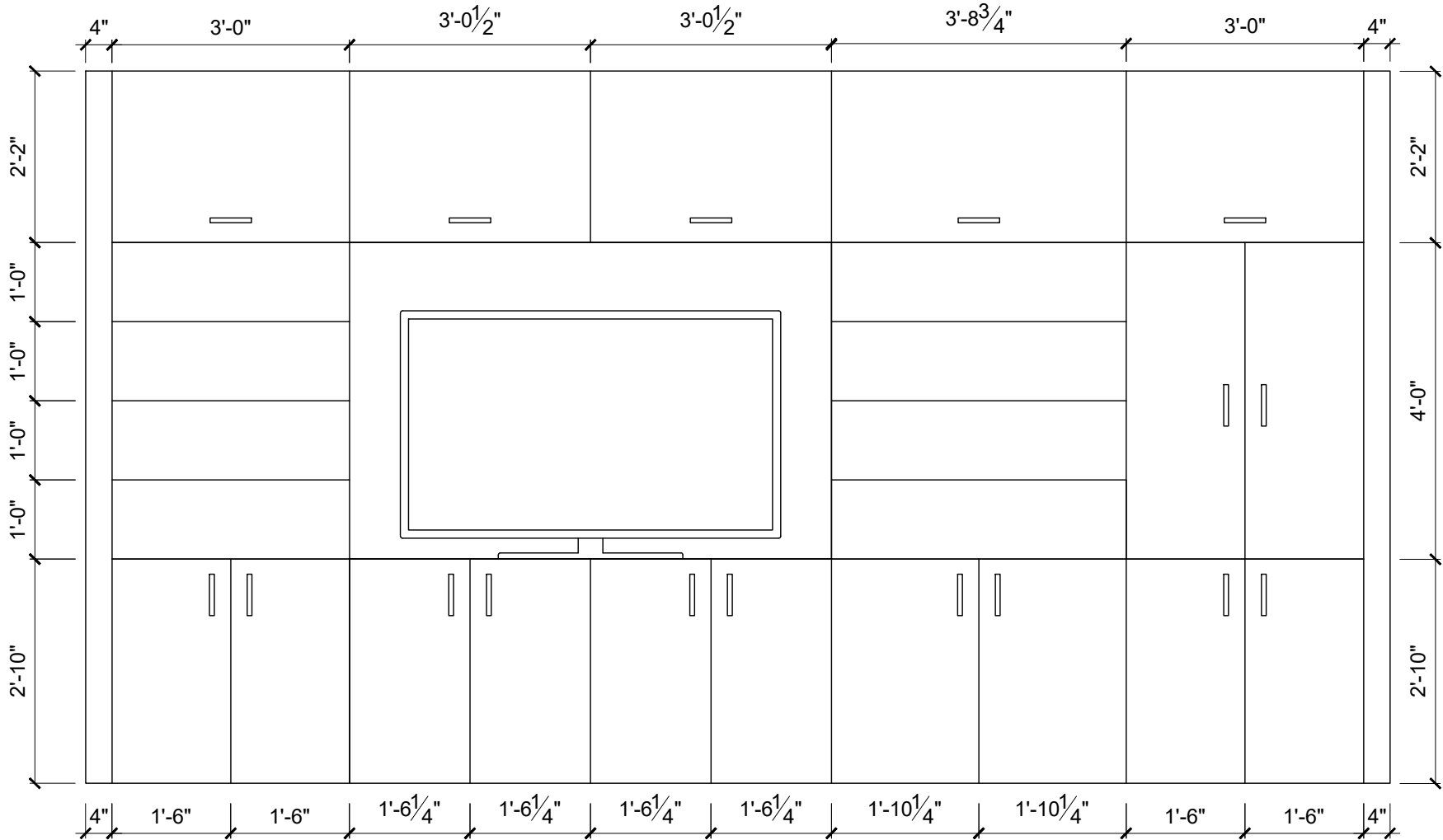
1 NEEL RESIDENCE - ELEVATION OF CUSTOM LIVING BUILT IN ID-7 SCALE: 1/2" = 1'-0"
